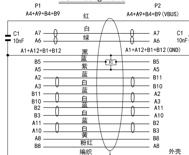
PIN Assignment
